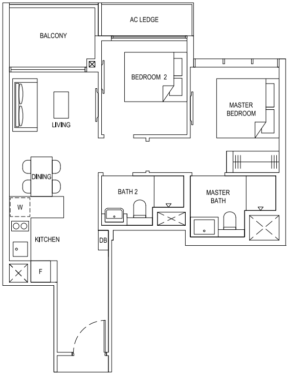
TYPE 2D3(G) 62 sqm / 667 sqft
