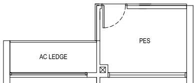
TYPE 1B1(G) 44 sqm / 474 sqft #01-57 (BLOCK 93) #01-60* (BLOCK 93)
